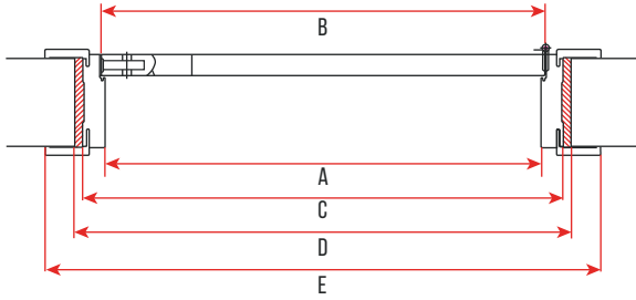
RESİM/PICTURE 1: KAPI GENEL KESİT DOOR'S GENERAL CROSS SECTION
